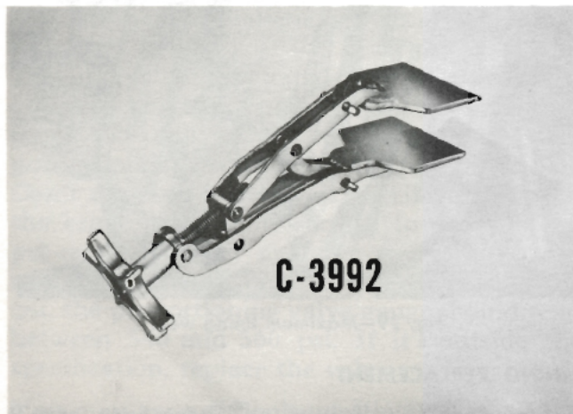
Fig. 31—Forces pistons back into the bores
