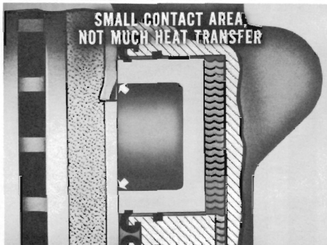
Fig. 11—Hollow pistons don't conduct heat
