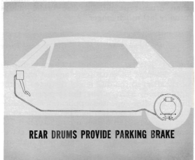
Fig. 3—Drum brakes for parking
