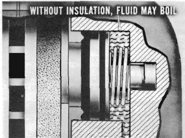
Fig. 26—Insulator keeps the piston cool
