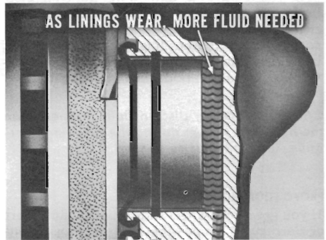
Fig. 21—Fluid level should be checked often
