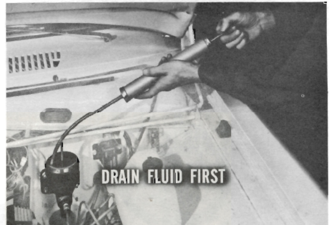
Fig. 22—Make room for fluid in the calipers
