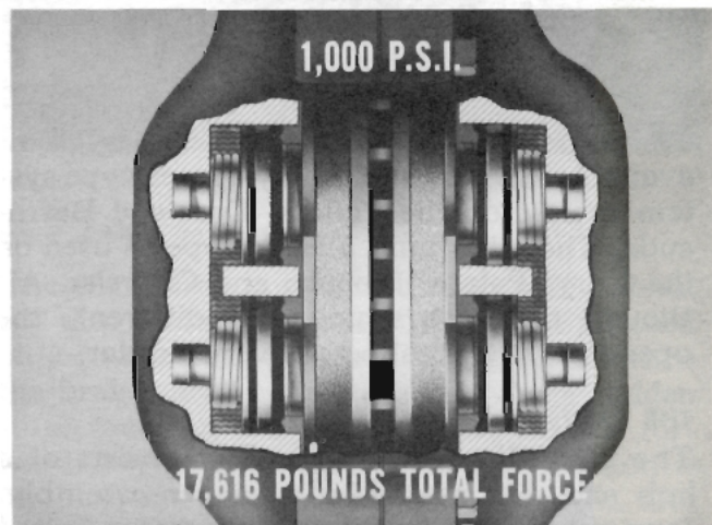
Fig. 7—More force for same pressure
