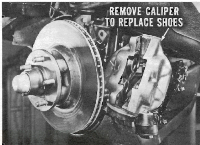
Fig. 30—It's not necessary to open hydraulic lines
