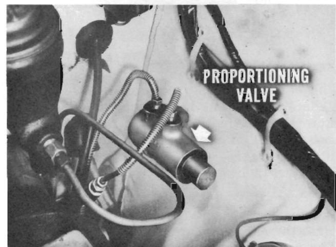
Fig. 13—Valve limits rear cylinder pressure
