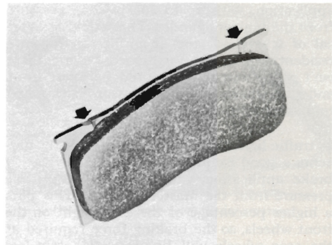
Fig. 19—Tabs signal worn out shoes
