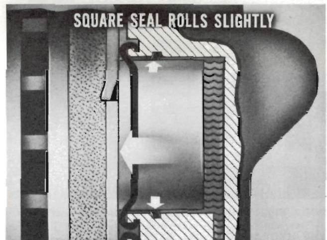
Fig. 9—The piston rolls the seal
