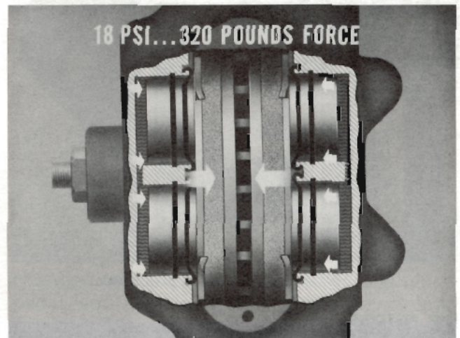
Fig. 8—Residual pressure would cause drag
