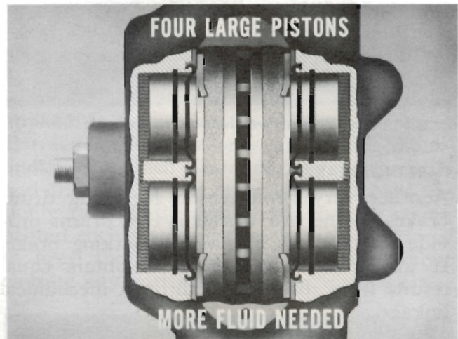
Fig. 6—Higher fluid requirements
