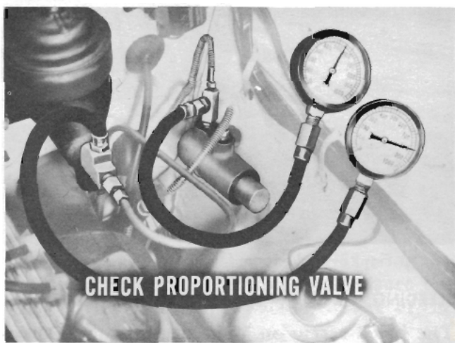
Fig. 24—Proportioning valve must reduce pressure
