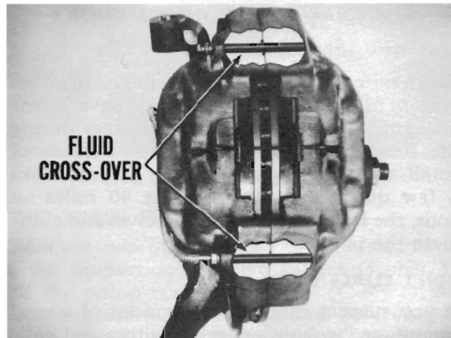
Fig. 27—Passage supplies fluid to outer-half
